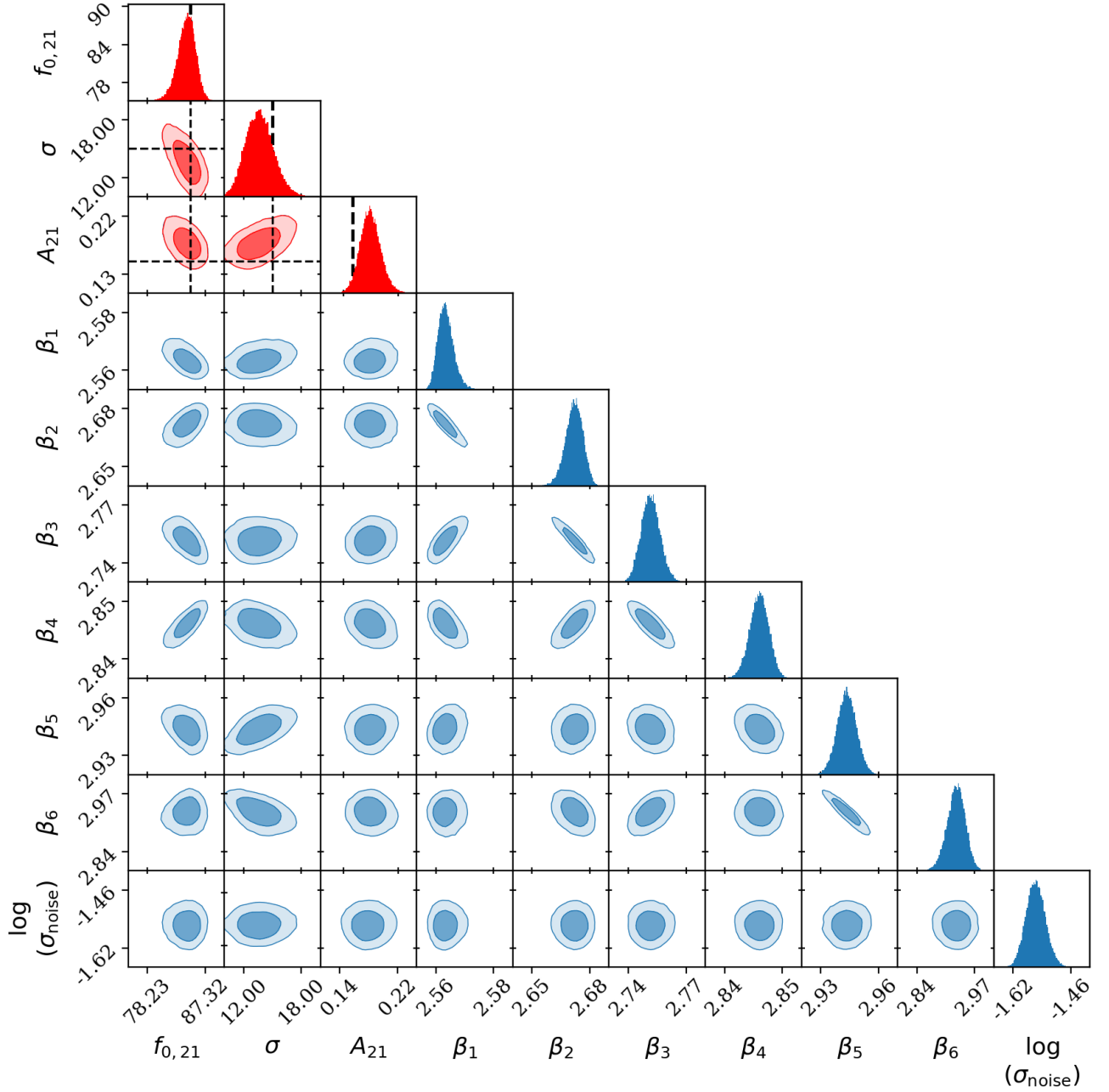
Figure A1. Corner plot of the posterior distributions for the SignalData/SignalFit case of the 4-hour Galactic integration using beam-nested sky partitioning with N_{\text{reg}} = 6 . Signal parameters are shown in red, including the 21-cm amplitude A_{21} , central frequency f_0 , and width \sigma , while foreground and noise parameters are shown in blue, including the spectral indices \beta_1, \dots, \beta_6 and the noise amplitude, \log(\sigma_{\text{noise}}) . Diagonal panels show one-dimensional marginalised posteriors, and lower-triangle panels show the two-dimensional posterior structure estimated via kernel density estimation. Black dashed lines mark the injected fiducial signal parameter values ( A_{21} , f_0 , \sigma ) for reference. Generated using the anesthetic package (Handley 2019).
