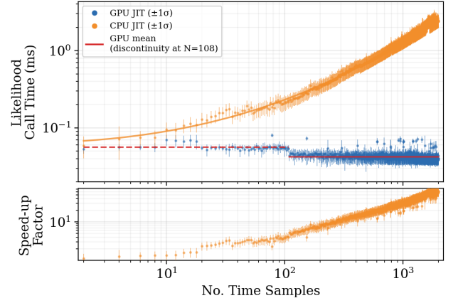
Figure 5. Performance benchmarking of the likelihood evaluation across varying data volumes. Top: Comparison of mean execution time (ms) for 1000 likelihood calls on an Intel Cascade Lake CPU (with JIT compilation) versus an NVIDIA A100 GPU, with discontinuity highlighted in by red line (dashed/solid). Bottom: The resulting speed-up factor of the A100 implementation relative to the JIT CPU baselines.
