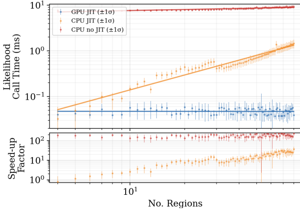
Figure 4. Performance benchmarking of the likelihood evaluation across varying model complexities. Top: Comparison of mean execution time (ms) for 1000 likelihood calls on an Intel Cascade Lake CPU (with and without JIT compilation) versus an NVIDIA A100 GPU. Bottom: The resulting speed-up factor of the A100 implementation relative to both JIT and non-JIT CPU baselines.
