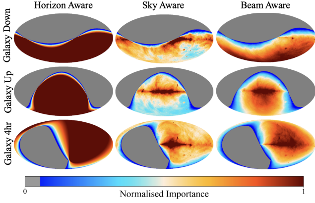
Figure 6. Time-integrated importance maps in Galactic coordinates used to construct sky regions. Each row corresponds to an observing window: Galaxy Down (1hr), Galaxy Up (1hr) and a 4hr Galaxy integration, and each column shows a different weighting: “horizon aware” (visibility-only), “sky aware” (sky-brightness-weighted), and “beam aware” (beam-convolved sky-brightness-weighted). Colours indicate relative importance, with higher-importance regions shown in red, lower-importance regions in blue, and grey indicating zero weight. The beam-aware maps concentrate weight where the instrument is both sensitive and the sky is bright, producing observation-dependent importance structures that motivate adaptive region definitions for foreground parametrisation.
