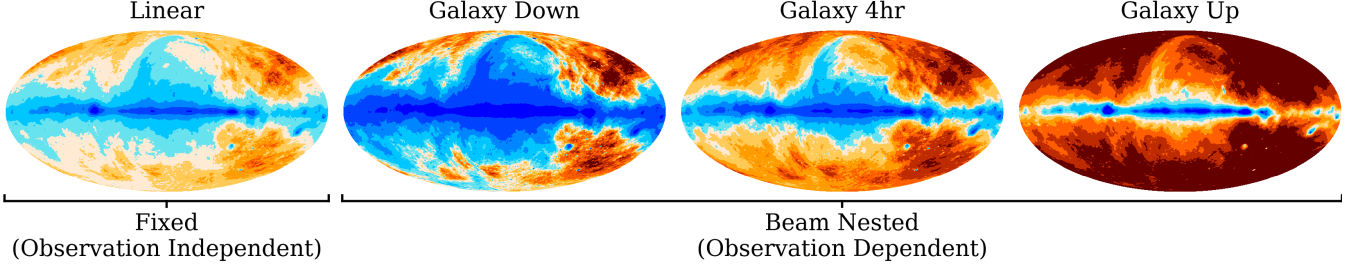
Figure 9. Comparison of discrete sky splitting masks M_{\beta,j} for N_{\text{reg}} = 11 regions in Galactic coordinates. The columns compare an observation-independent linear splitting baseline with observation-dependent ‘beam-weighted’ recursive splitting schemes for three observing windows: Galaxy Down (1 hr), Galaxy Up (1 hr), and a 4-hr Galaxy integration, with each colour representing a unique binary mask M_{\beta,j} . The adaptive scheme allows region boundaries to be redistributed to prioritise finer resolution in areas where the beam-convolved sky-brightness is highest.
