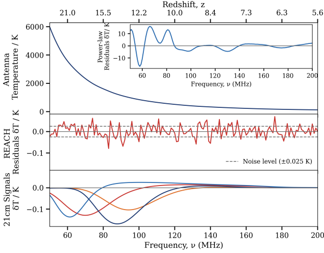
Figure 2. A demonstration of the chromatic structure introduced by the coupling of the Galactic foregrounds and the beam, its degeneracy with global 21-cm signals, and how these effects can be accounted for with the REACH data analysis pipeline. Top panel: A simulated 1 hour time-averaged observation d(\nu) from the REACH telescope in the Karoo Desert, South Africa at 00:00 01-10-2019 with a conical log spiral antenna. The data has a mock 21-cm signal and 0.025 mK of Gaussian noise injected. The inset shows residuals beyond a fitted smooth power-law. Middle panel: Reduced residual structure after subtracting a Bayesian nested sampling fit model produced by the REACH pipeline using 16 parametrised regions. Bottom panel: Examples of emulated mock signals from GlobalEMU (Bevins et al. 2021b), to demonstrate the success of beam-aware modelling suppressing residuals below the magnitude of expected global 21-cm signal.
