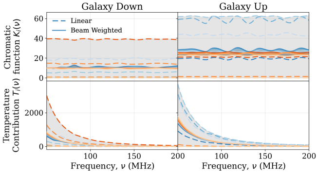
Figure 8. A comparison of the chromatic response tensors and spectral index scaled antenna temperature for 8 regions defined using linear versus beam-hierarchical sky splitting schemes. The columns show unique observing windows: Galaxy Down and Galaxy Up. Top row: chromaticity functions K_i(\nu) for each region, shown for an observation-independent linear split (dashed) and an observation-dependent beam-hierarchical split (solid). Bottom row: corresponding region contributions T_i(\nu) after applying assigned spectral-index scaling. The range of magnitudes/ contributions across all regions is demonstrated by the min/max shading for linear (light grey) and beam hierarchical (dark grey).
