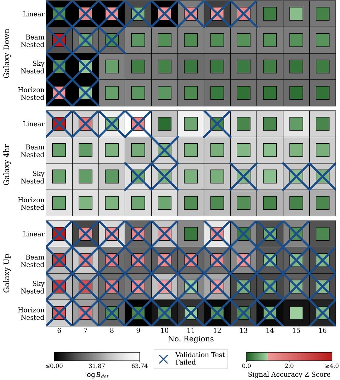
Figure 13. Summary of signal recovery and Bayesian model selection across sky-splitting methods and region counts. Each panel corresponds to a unique observing window, with columns indicating the number of regions ( N_{\text{reg}} = 6\text{--}16 ) and rows showing the different sky-splitting schemes. The outer shaded square encodes the Bayesian evidence in favour of a signal detection, quantified by the log Bayes factor \log B_{\text{det}} , with lighter colours indicating stronger support for the signal model. The inner square displays the statistical consistency of the recovered posterior with the injected signal via the Z-score, shown using a green-to-red colormap. Validation failures are indicated by a single blue cross, drawn when either the null test (signal preferred in no-signal injections) or the residual consistency test fails, signalling potential residual systematics degenerate with the global 21-cm signal.
