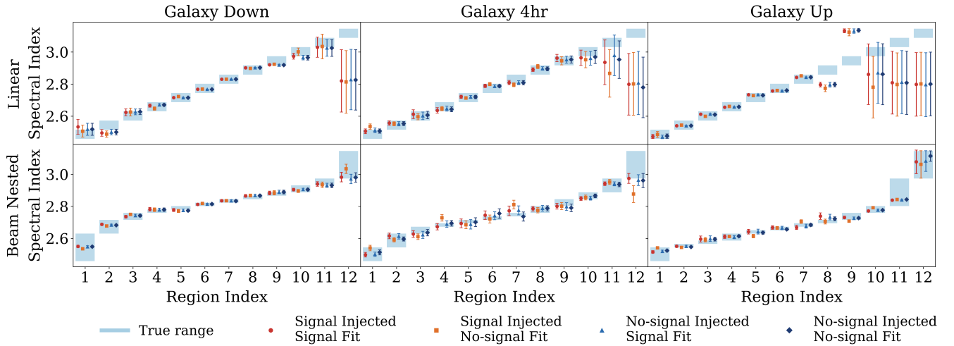
Figure 12. Comparison of foreground spectral index recovery using linear vs. beam-nested sky parameterisation schemes ( N_{\text{reg}} = 12 ). Columns represent different observing windows (Galaxy Down, Galaxy Up, and a 4 hr Integration), while rows compare the linear splitting method (top) with the beam-nested splitting method (bottom). In each panel, the shaded bands indicate the ground-truth range of spectral indices ( \beta ) present within that specific region on the high-resolution ( N_{\text{side}} = 512 ) base map used for data generation. The overlaid points and 1\sigma error bars show recovered posterior means for the four generation/fit combinations (Signal Injected/Signal Fit, Signal Injected/No-signal Fit, No-signal Injected/Signal Fit, No-signal Injected/No-signal Fit).
